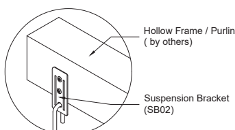
ANCHORAGE TO HS / PURLIN - OPTION 1
