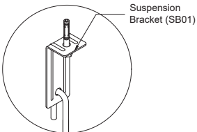
ANCHORAGE TO SOFFIT - OPTION 1
