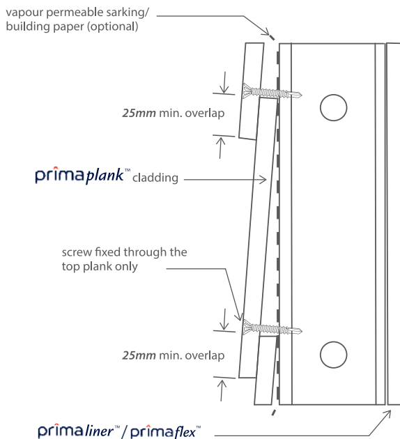
Figure 3.8: Fastening to steel frame
