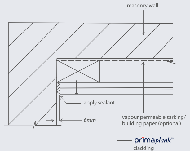
Figure 2.5.1: Jointing with other material
