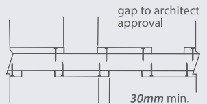
Horizontal Section
