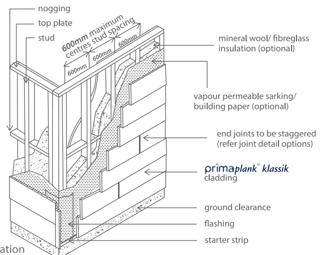
Figure 3.2.1: Horizontal planking
