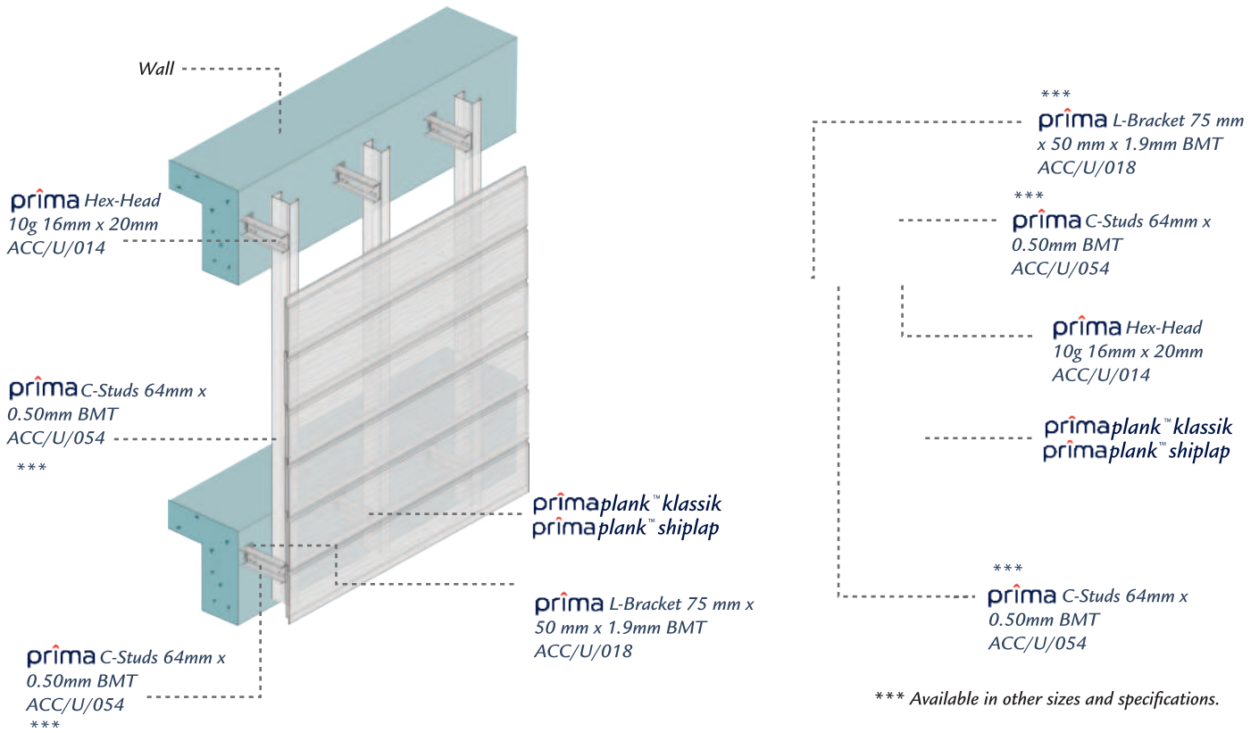
Figure 3.2.3: Cantilever Cladding System
