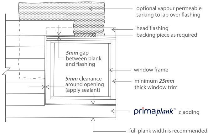
Figure 3.12.1: Window/ door opening detail
