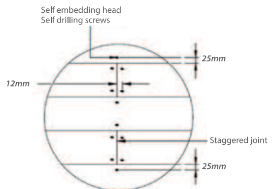
Figure 8.3.2: Fastener Fixing
