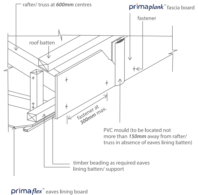
Figure 5.3: PVC joint
