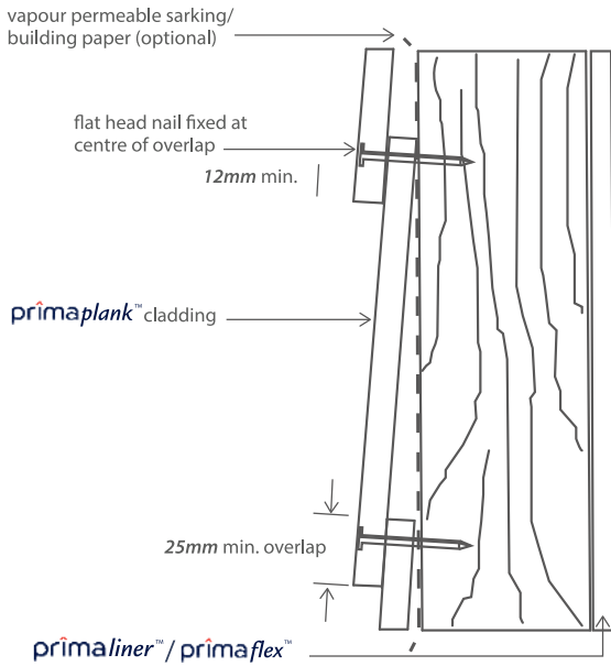
Figure 3.7: Fastening to timber frame
