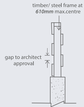
Horizontal Section
