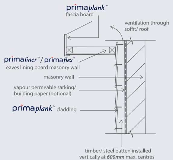
Figure 4.6: Wall ventilation detail
