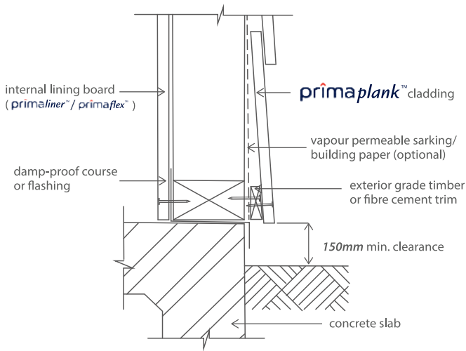
Figure 3.10: Ground Clearance
