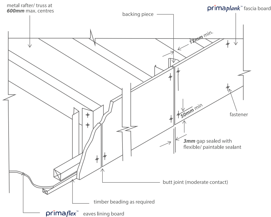
Figure 5.4: Butt joint & sealant (Metal rafter/ truss)
