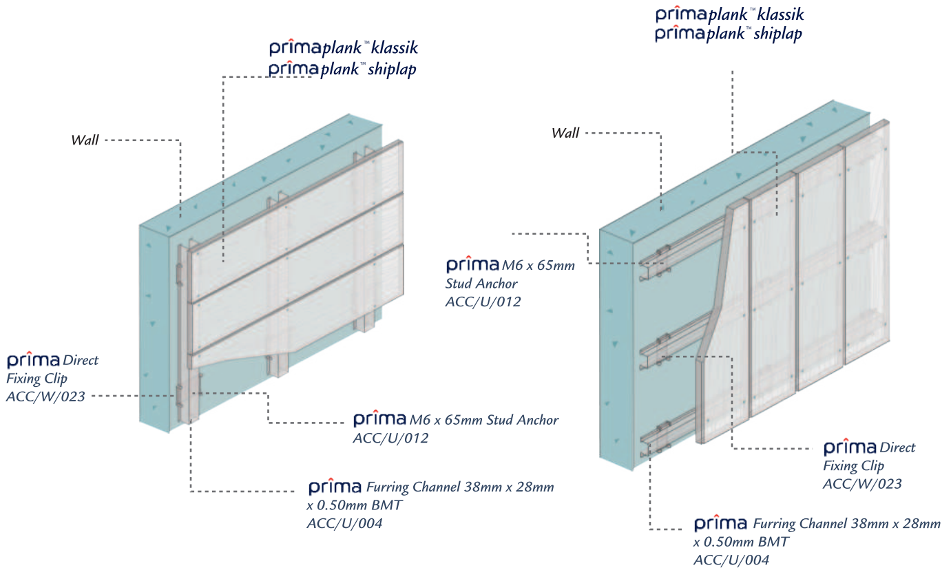
Figure 3.2.2: Direct Fixing Cladding System
