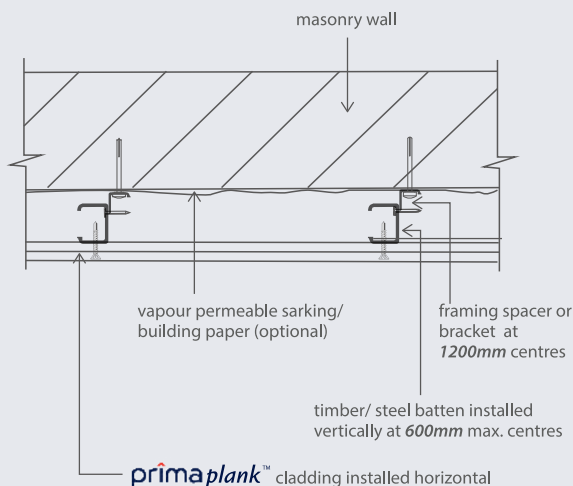
Figure 4.3.2: Battening onto uneven masonry wall
