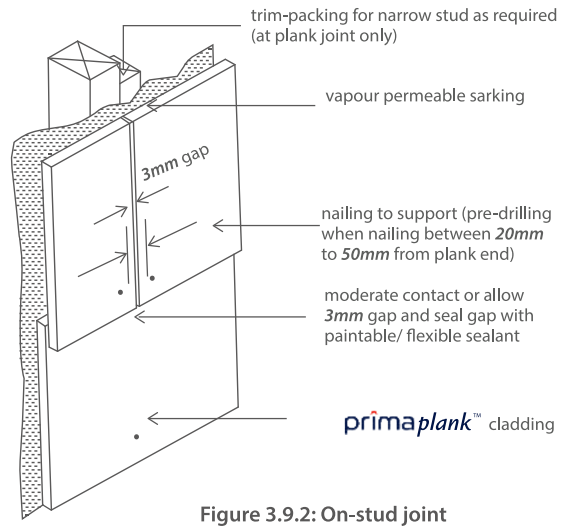
Figure 3.9.2: On-stud joint
