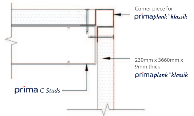
Figure 3.11.4: External corner solution corner piece
