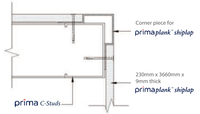
Figure 3.11.3: External corner solution corner piece
