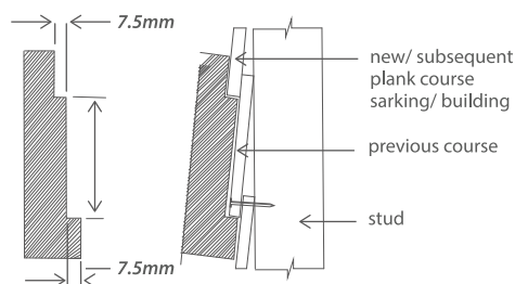
Figure 3.5: prima plank ™ Lap gauge
