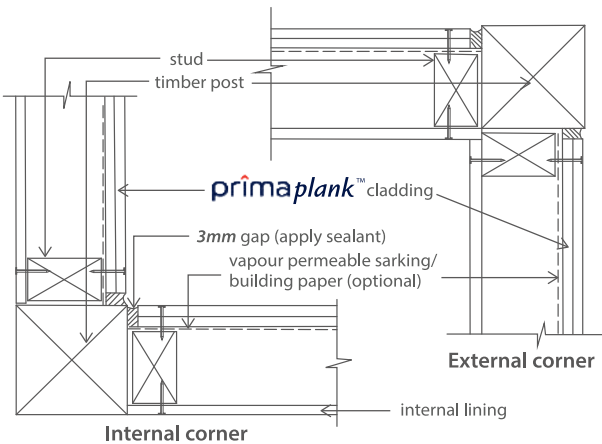
Figure 3.11.2: Timber post corners
