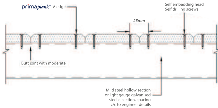
Figure 8.3.3: Joint Detail at along edges
