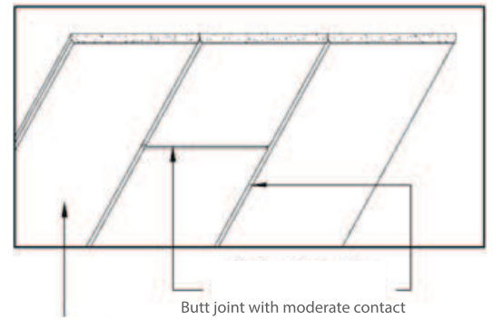
Figure 7.3.2: Joint Detail
