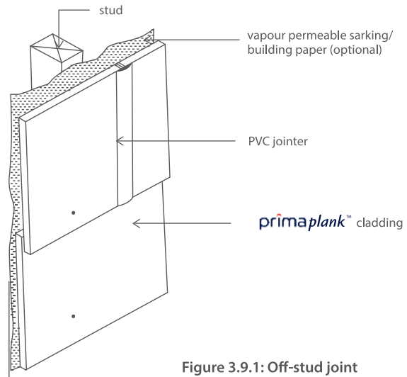
Figure 3.9.1: Off-stud joint
